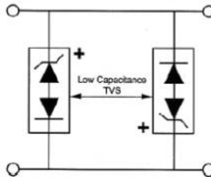
Fig. 4 - AC Line Protection Application
